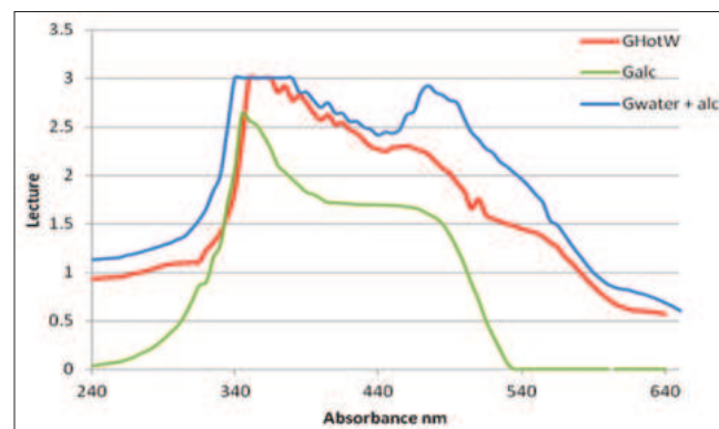
Fig 1. Spectrophotometer lectures (A240-660) from samples GHotW (extracted with hot water); GAlc (extracted with alcohol), GWater-Alc (extracted with hot water and mixture 20% of alcohol extract). Peaks observed: GWater-Alc 322, 390, 405, 415,425, 445, 475nm; GHotW 322, 350, 375, 385, 445-485, 510nm and GAlc 322, 435-485nm.
